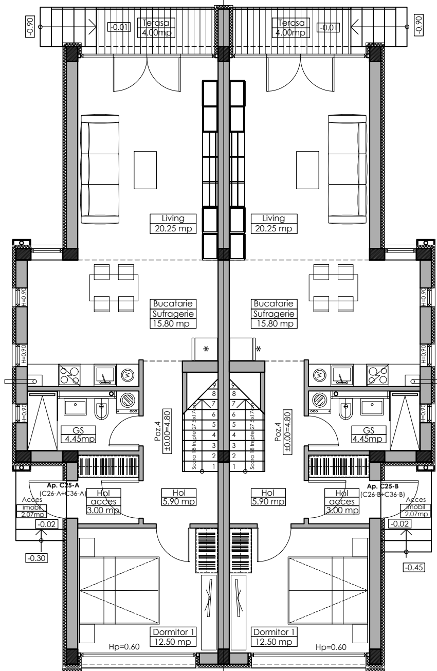
Parter_Poz.4 ÷15. Ap: C25-B ÷ C36-B 4 CAMERE
